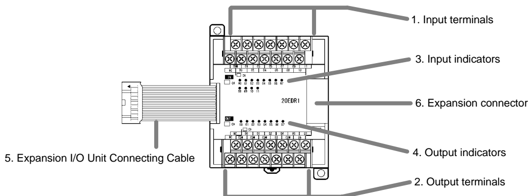
Expansion I/O Unit with 20 I/O Terminals
