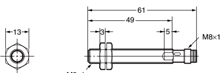
E2A-S08LS02-M5-□□
